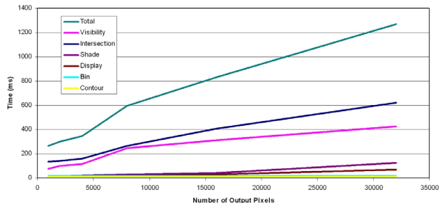
Figure 7 – A plot of the execution times for each step of the IBVH rendering algorithm on a single CPU. A typical IBVH might cover approximately 8000 pixels in a 640 \times 480 image and it would execute at greater than 8 frames per second on our 4 CPU machine.
